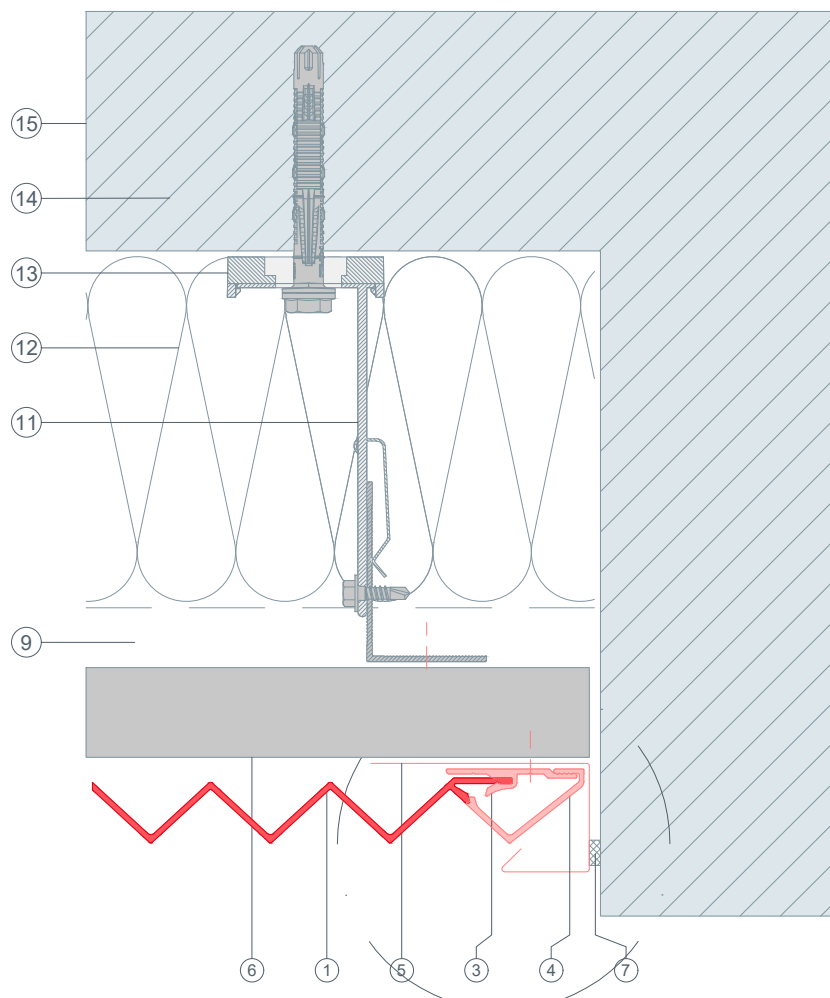
connection variant
