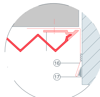
connection variant
